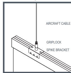
27mm Spike Bracket
